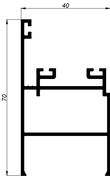
41002 MARCO LATERAL
