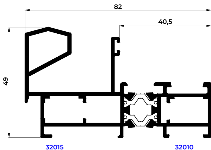
69005 MARCO MONOCARRIL
